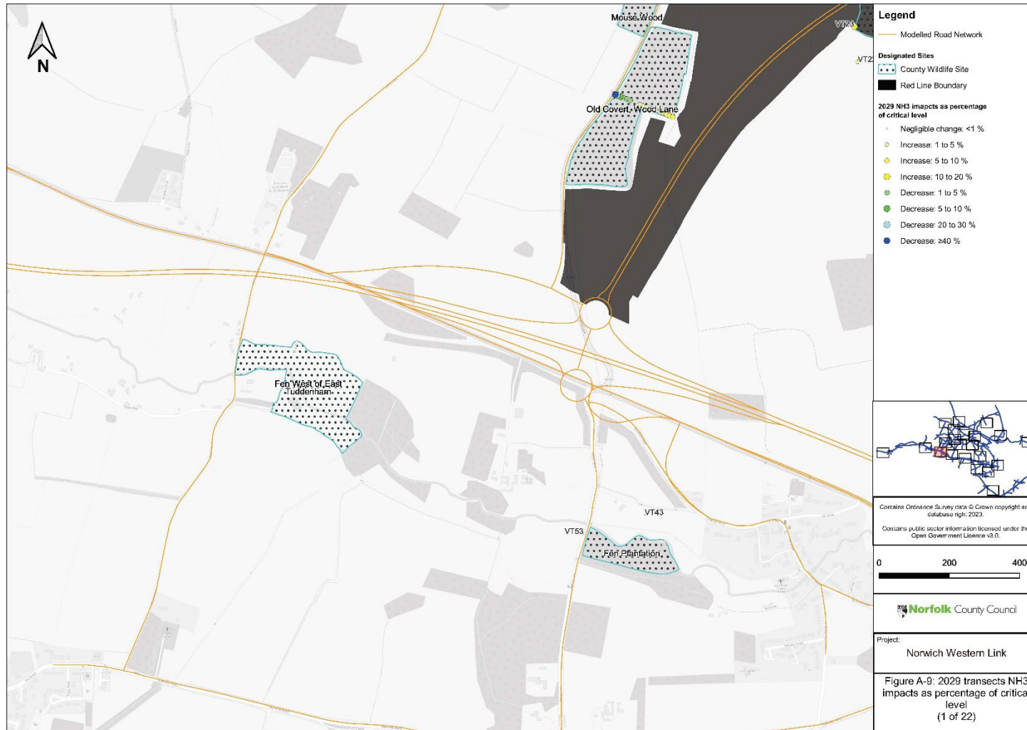
Figure A 9 2029 Transect NH3 Impacts as percentage of critical level
